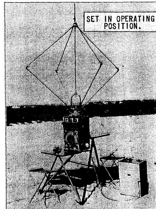
L. &amp; M.W. P/24b-313 (D/F RECEIVER)
