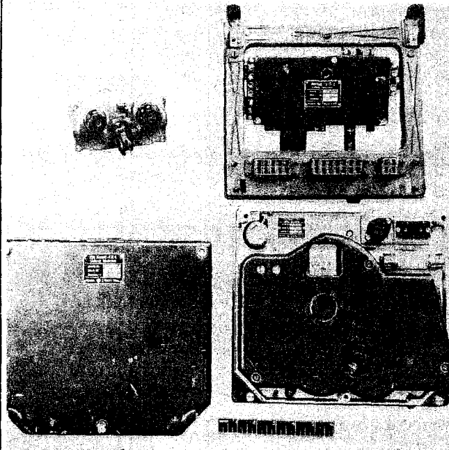
PEIL G 4 - RECEIVER EZ 4, COMPLETE.
